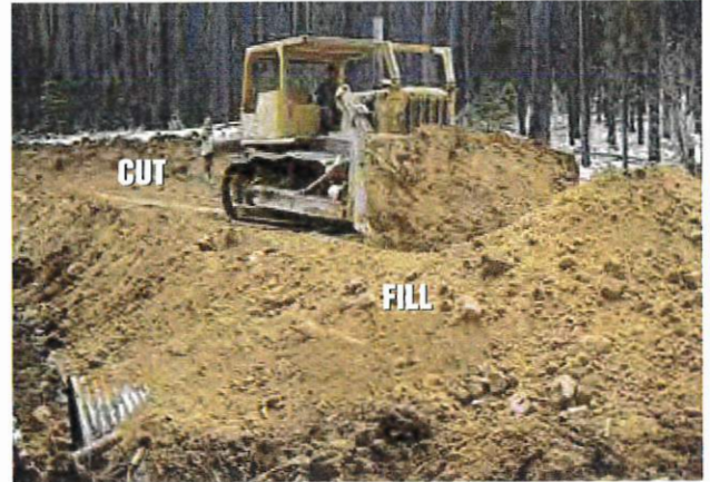
Cut-and-fill road construction is common for most terrain in Montana.
