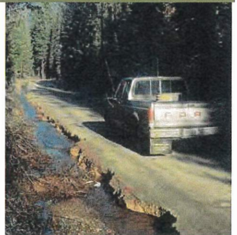
This plugged cross-drain culvert and washed-out catch basin can be a source of sediment.
