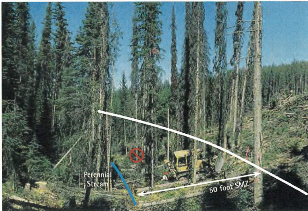
Directional falling and/or reaching into the SMZ with a mechanical feller-buncher allows removal of some SMZ trees without damaging the SMZ.
