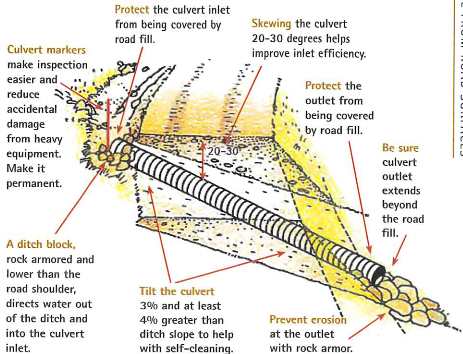
Mitered Relief Culvert Inlets can prevent plugging from soil or debris.
